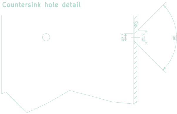
Countersink hole detail
